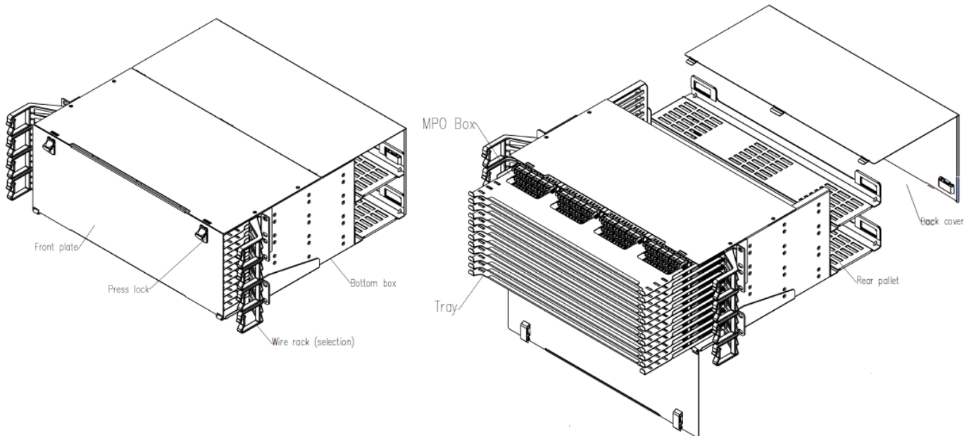
Figure 2. Giganet 4U 48 slots UHD Modular Sliding Patch Panel Technical Drawing
