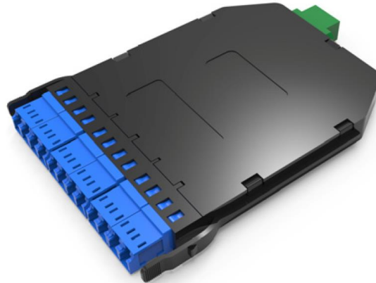
Figure 1. Giganet UHD-MTP/MPO Cassette Modules Base 12 (B)
