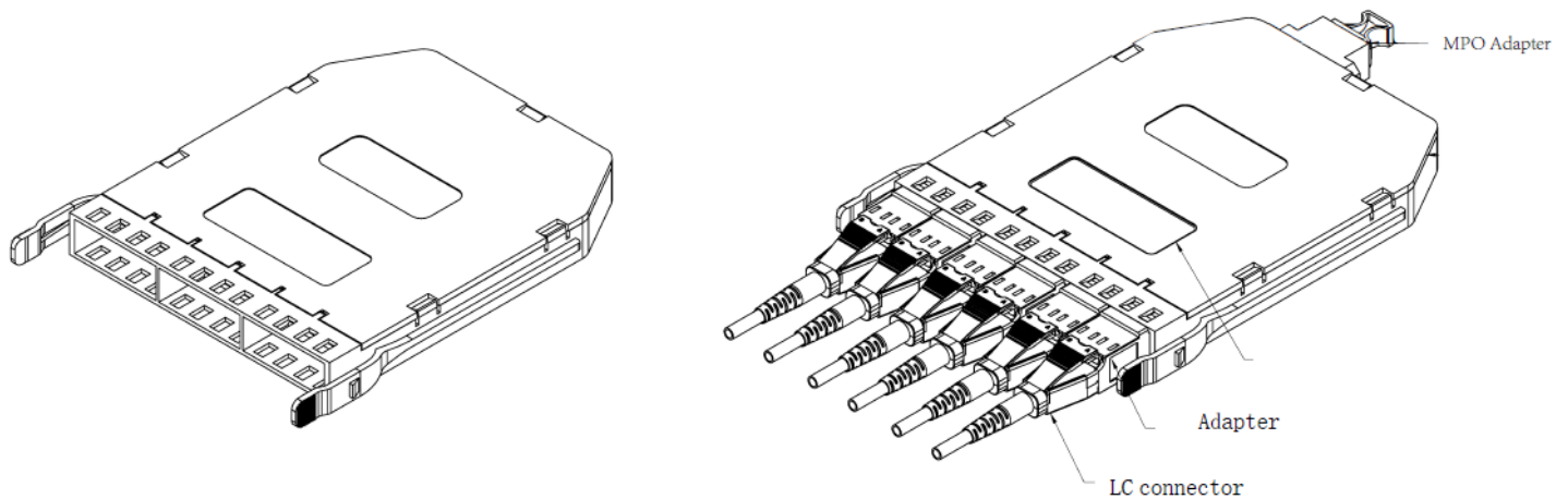
Figure 2. Giganet UHD-MTP/MPO Cassette Modules Base 12 (B) Technical Drawing
