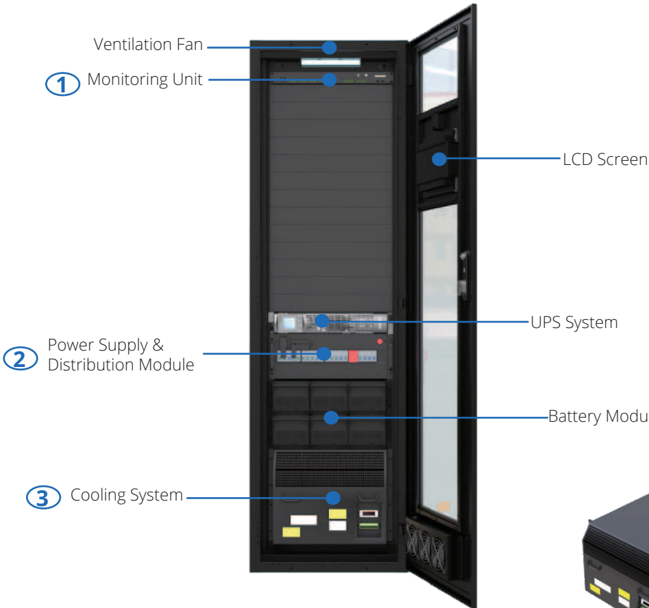
Monitoring Unit All in one monitoring host collects, displays and reports system status, locally and remotely.
