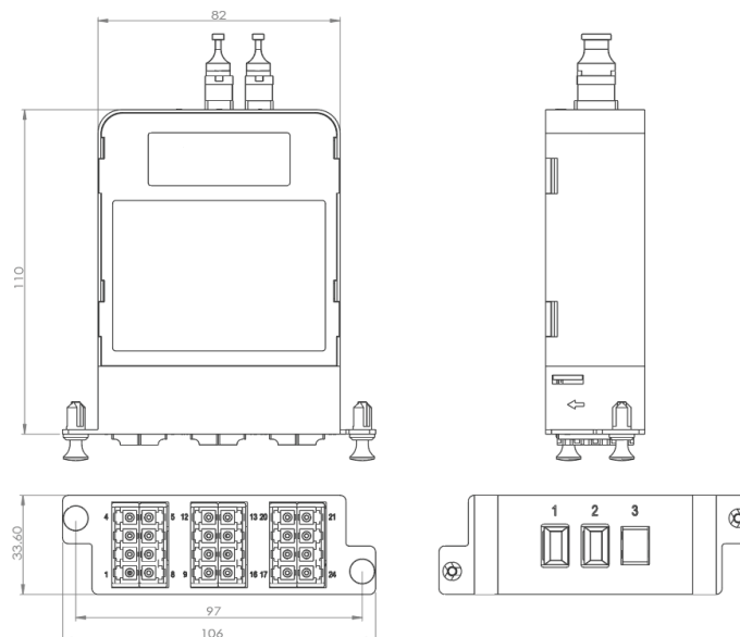
Figure 2. Giganet HD-MTP/MPO Cassette Modules Base 12 (A and C) Technical Drawing
