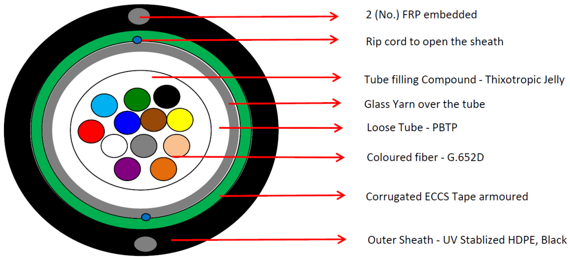
Cable Cross Sectional Diagram of 12F Cable [Drawing not to scale]
