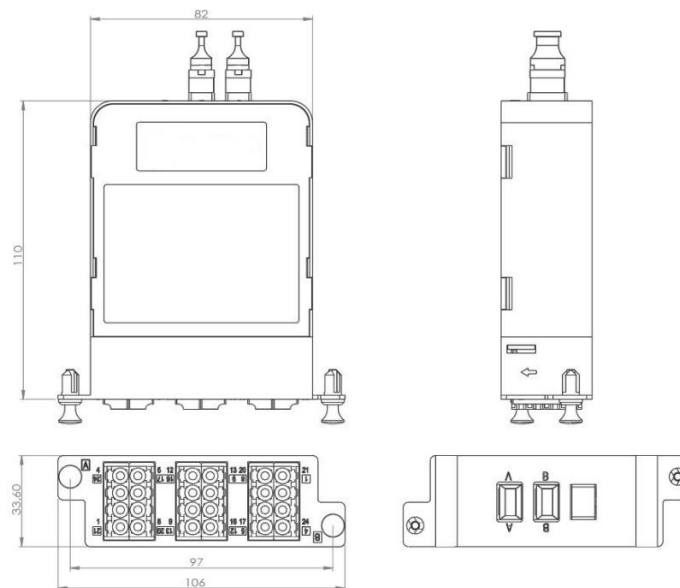
Figure 2. Giganet HD-MTP/MPO Cassette Modules Base 12 (Type B/Universal) Technical Drawing
