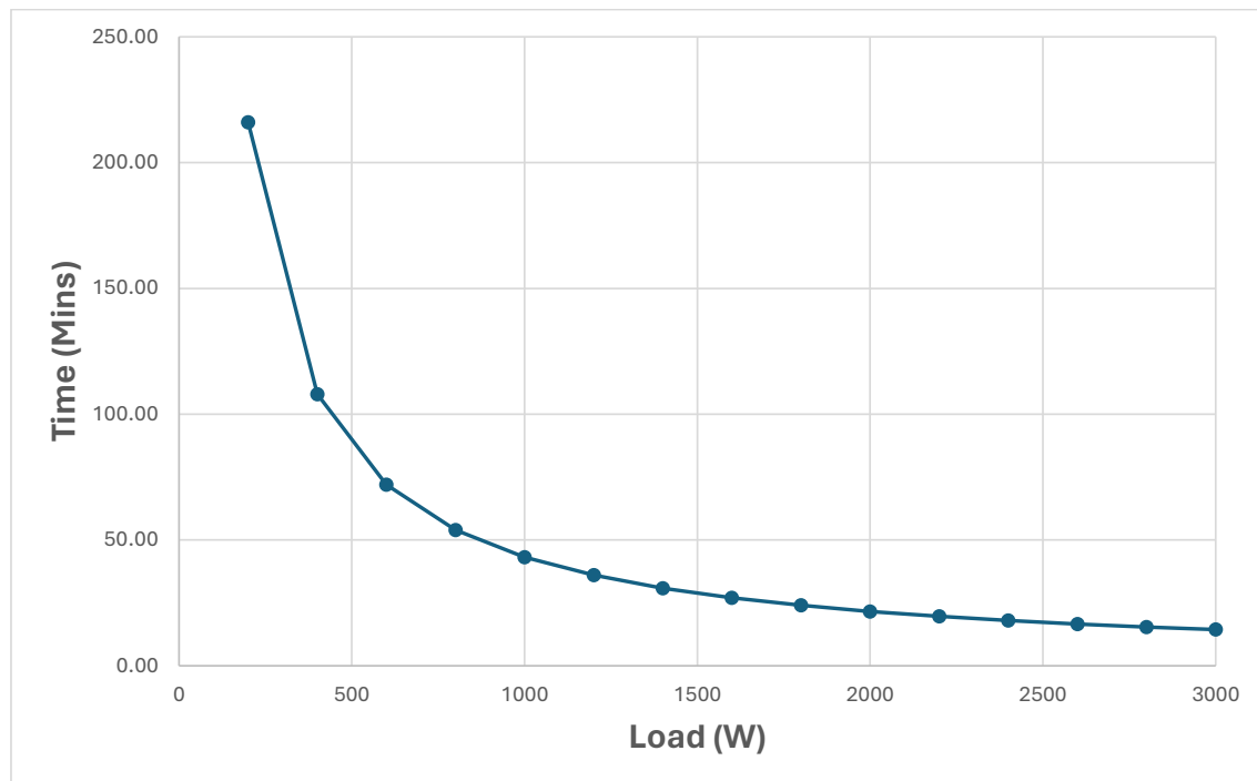
Runtime for Giganet UPS Online Double Conversion 3000VA UPS, with 6xIEC C13 Power Outlets and 1xIEC C19
