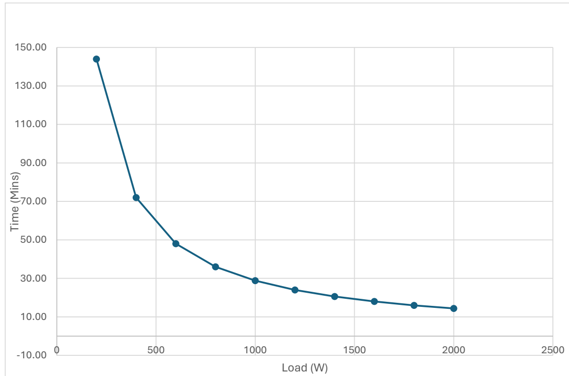
Runtime for Giganet UPS Online Double Conversion 2000VA UPS, with 6xIEC C13 Power Outlets
